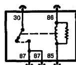
CONTACT RELAY WITH TWO OUTPUTS
