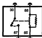
RELAY WITH RESISTOR ACROSS WINDING
