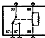
CHANGEOVER RELAY WITH TWO OUTPUTS
